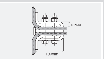
Supergrip No.4 > Belt Strength - 1250kN/m max. > Weight - 1.83Kgs > M16 Bolts
